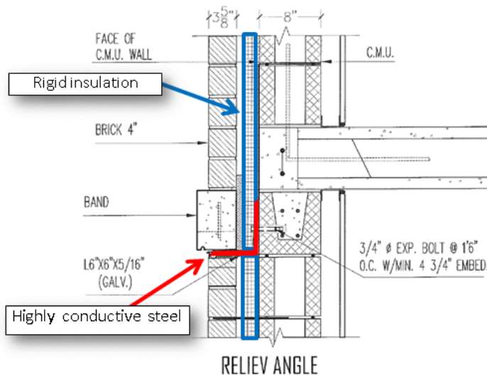
Figure 1: Wall construction utilizing shelf angle
